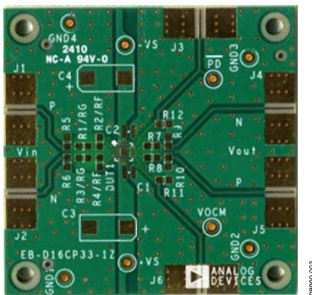
Figure 1. Component Side (LFCSP)
