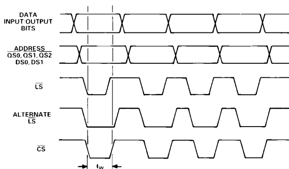
Figure 14. Load and Update Multiple DACs
