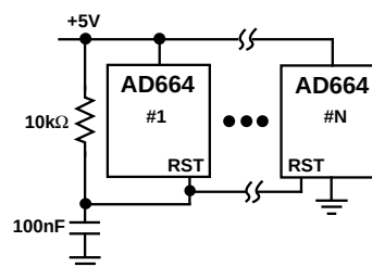
Figure 24. Power-On Reset
