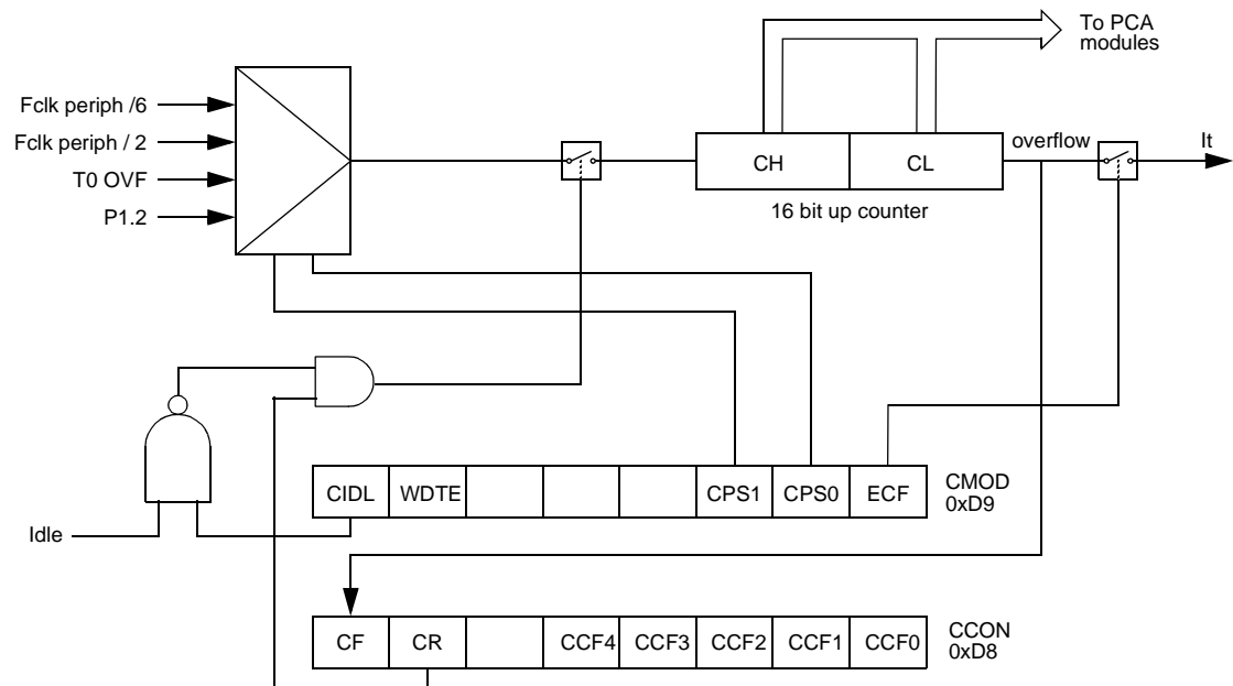
Figure 11. PCA Timer/Counter
