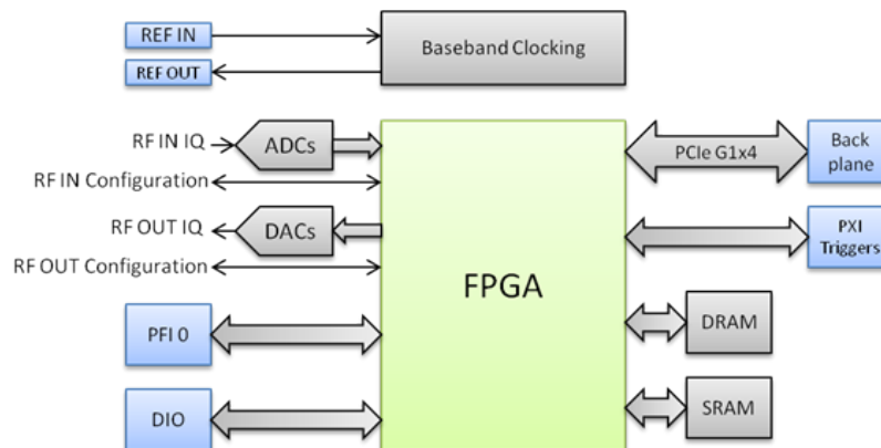
Figure 3. Block Diagram of the NI PXIe-5644R FPGA Basecard
