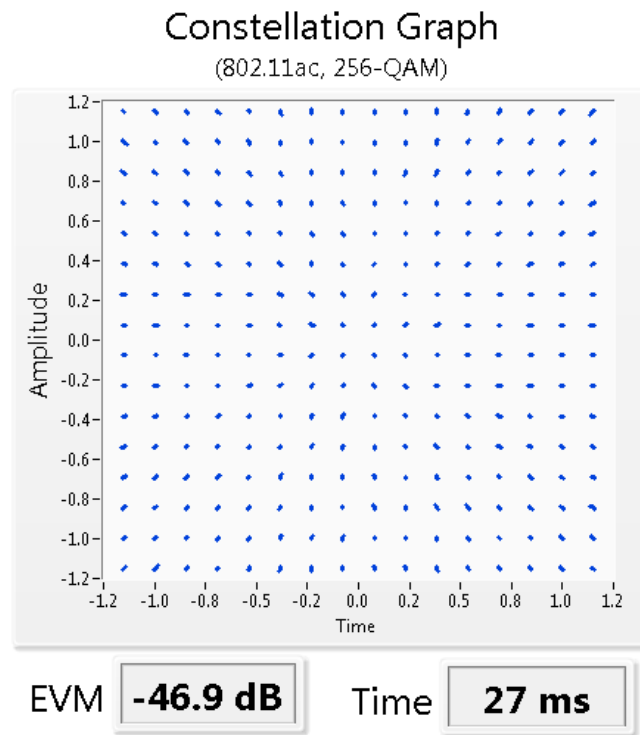
Figure 2. Typical Constellation Graph, EVM Measurement, and Measurement Time of an 802.11ac MCS9 Signal at 5.8 GHz.
