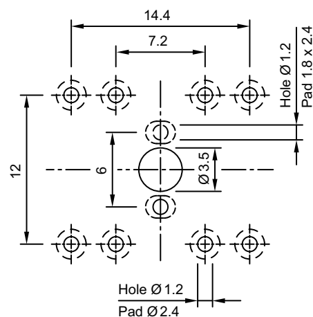
Drilling plan (Elementside) Through-connection recommended
