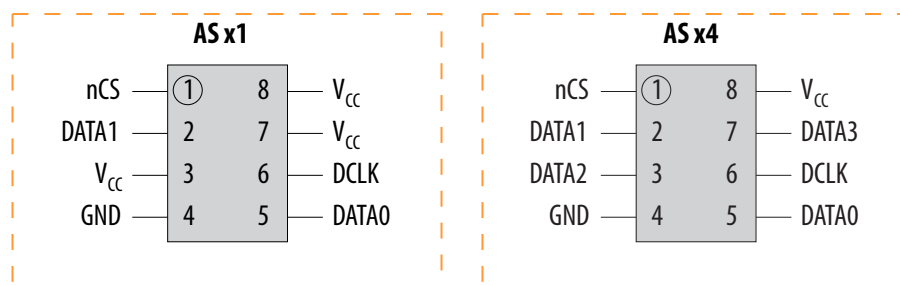
Figure 23. AS x1 and AS x4 Pin-Out Diagrams for EPCQ16 and EPCQ32 Devices
