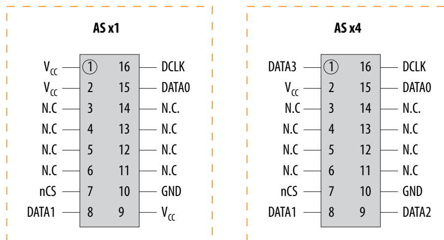
Figure 24. AS x1 and AS x4 Pin-Out Diagrams for EPCQ64, EPCQ128, EPCQ256, and EPCQ512/A Devices
