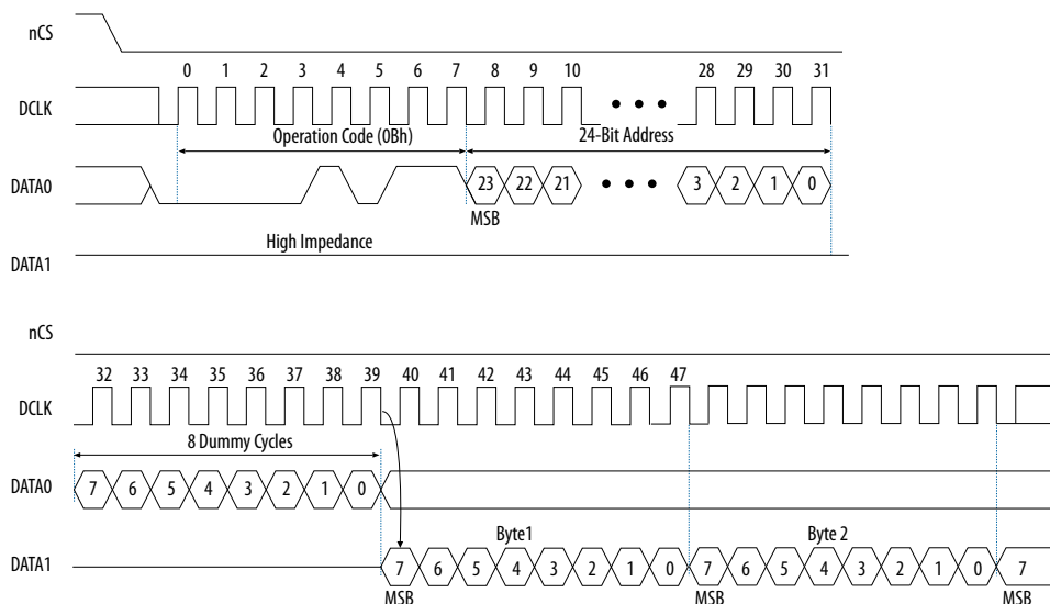
Figure 10. Fast Read Operation Timing Diagram
