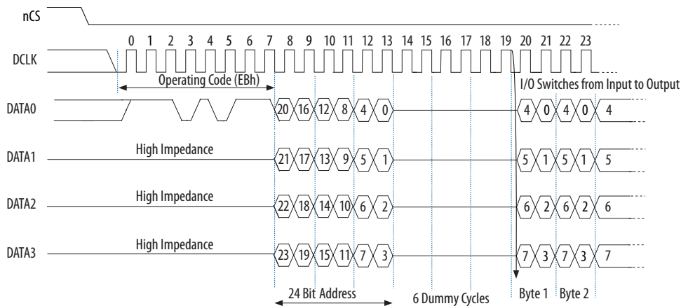
Figure 12. Extended Quad Input Fast Read Operation
