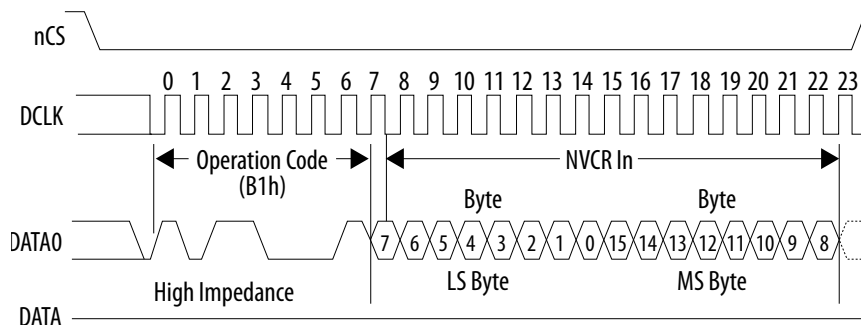
Figure 4. Write Non-Volatile Configuration Register Operation Timing Diagram
