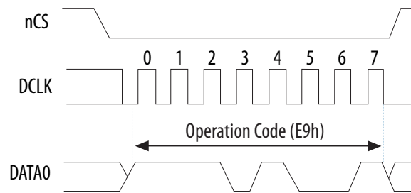
Figure 6. 4BYTEADDREX Timing Diagram
