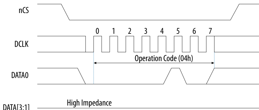
Figure 8. Write Disable Operation Timing Diagram
