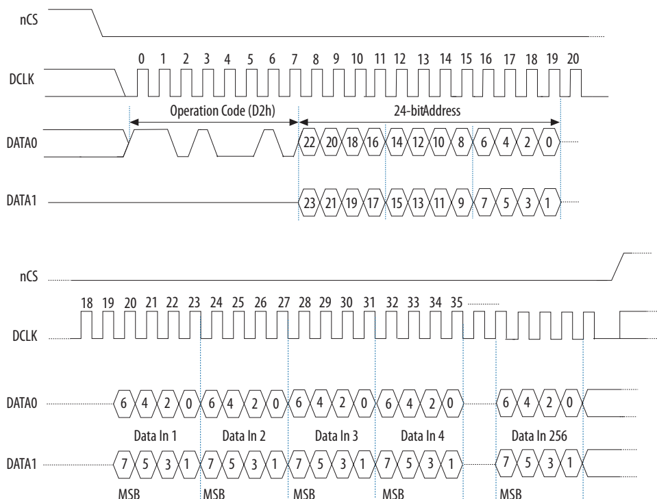
Figure 15. Extended Dual Input Fast Write Bytes Timing Diagram
