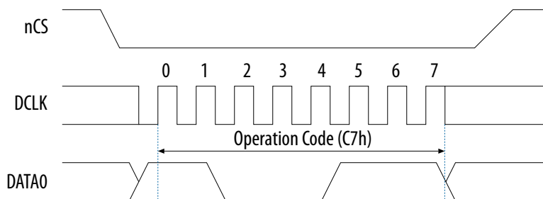
Figure 18. Erase Bulk Operation Timing Diagram
