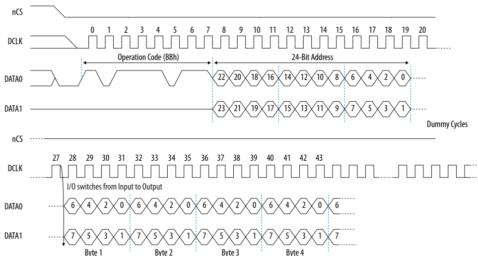
Figure 11. Extended Dual Input Fast Read Operation Timing Diagram
