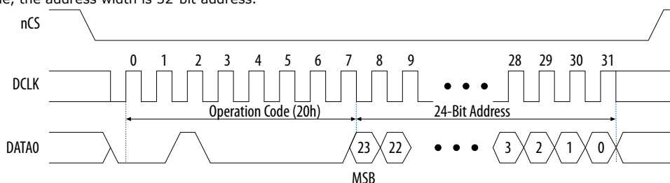
Figure 20. Erase Subsector Operation Timing Diagram
