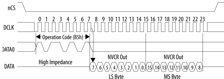
Figure 3. Read Non-Volatile Configuration Register Operation Timing Diagram
