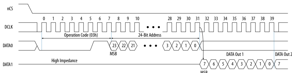
Figure 9. Read Bytes Operation Timing Diagram
