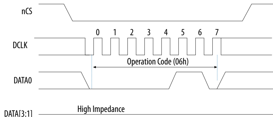
Figure 7. Write Enable Operation Timing Diagram
