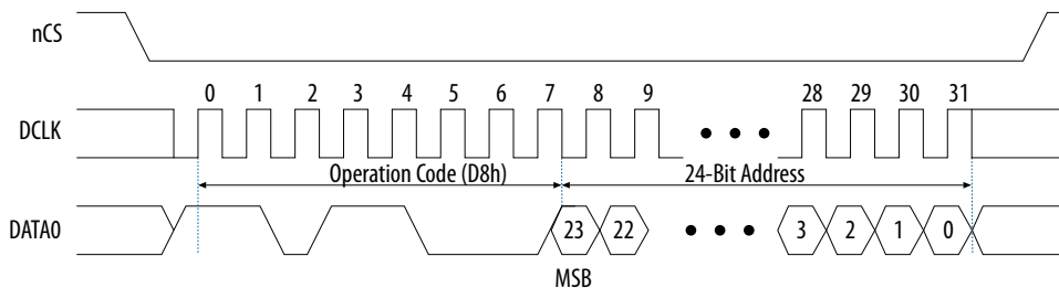
Figure 19. Erase Sector Operation Timing Diagram
