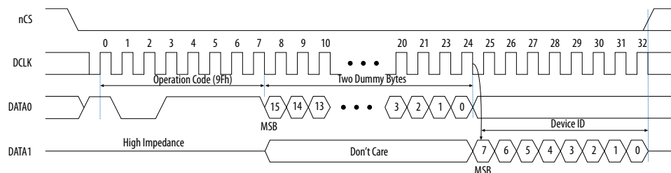
Figure 13. Read Device Identification Operation Timing Diagram
