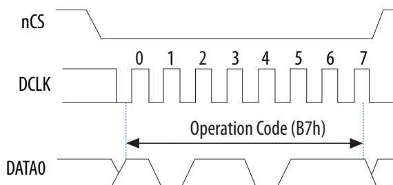
Figure 5. 4BYTEADDREN Timing Diagram
