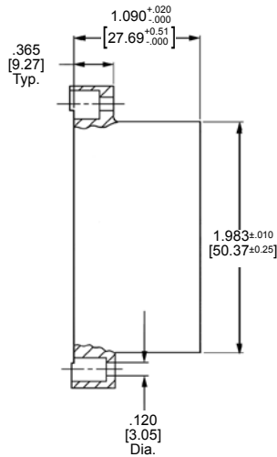
Plug Housing
