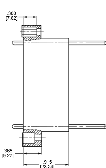
Plug Assembly (With Posted Pin Contacts)
