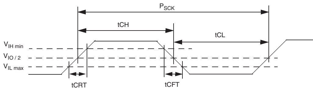
Figure 6.8 Clock Timing
