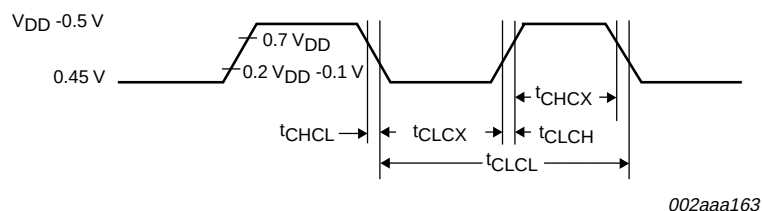
Fig 12. Clock signal waveform for I CC tests in active and idle modes (t CLCH = t CHCL = 5 ns).
