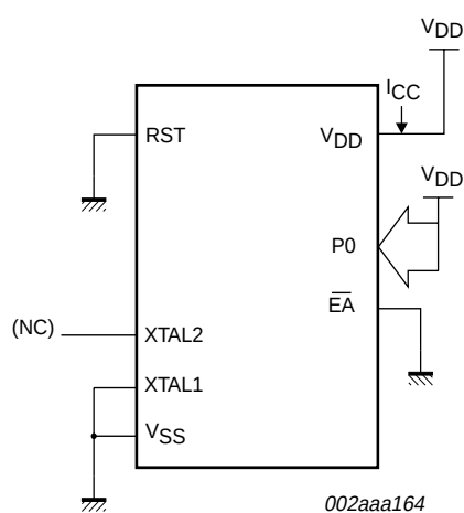
Fig 13. I CC test condition, power-down mode (all other pins are disconnected, V DD = 2.0 V to 5.5 V).
