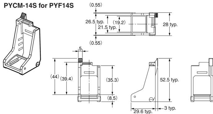
PYCM-14S for PYF14S
