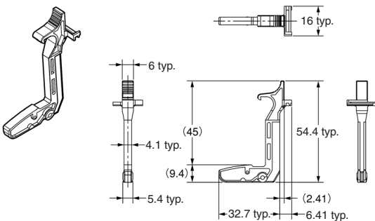
PYCM-08S for PYF08S
