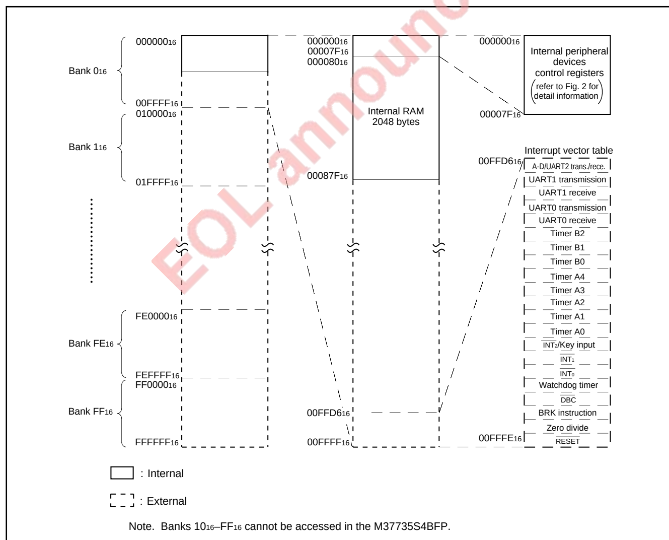
Fig. 1 Memory map
