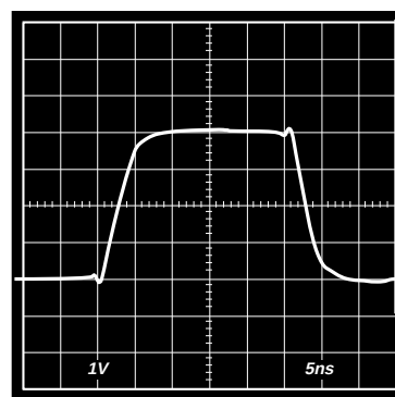
Figure 1. AD8047 Large Signal Transient Response, V_O = 4\text{ V p-p} , G = +1
