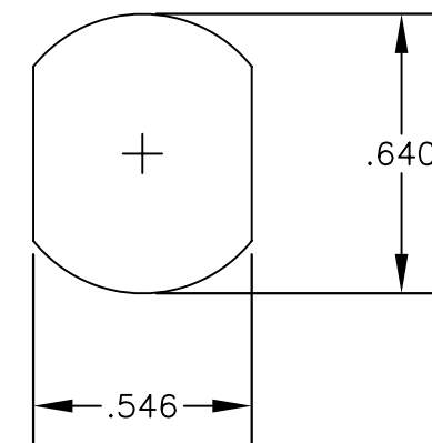
MOUNTING HOLE
