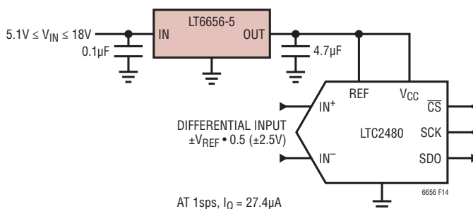
Figure 14. Low Power ADC Reference
