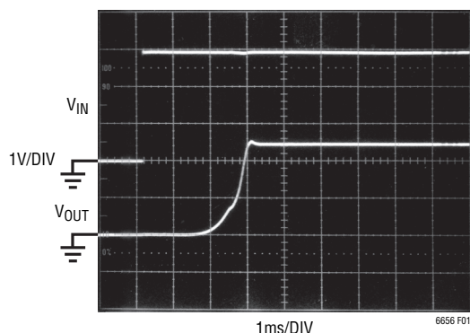
Figure 1. LT6656-2.5 Turn-On Characteristics, C_L = 1\mu F
