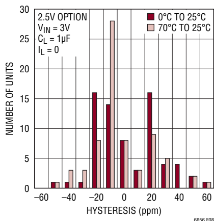
Figure 8. 0°C to 70°C Hysteresis
