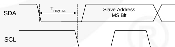
Figure 20. Start Bit
