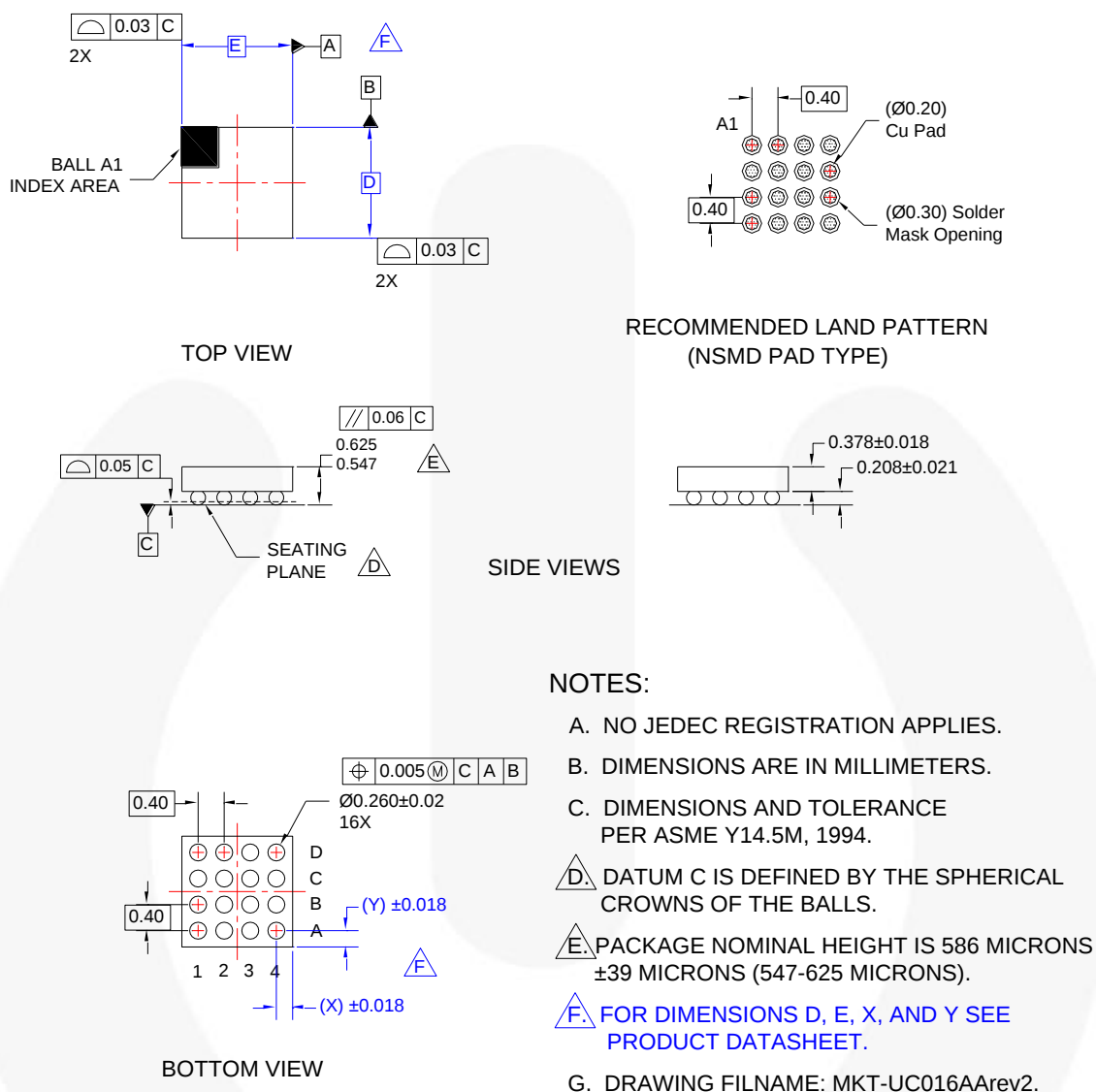
Figure 25. WLCSP-16, 0.4mm Pitch, Dimensions
