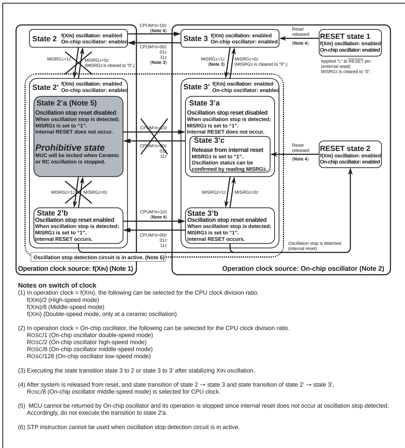
Fig. 84 State transition 2
