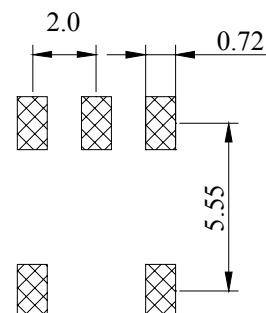
( PCB Pattern )
