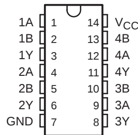
SN54LV00 ... J OR W PACKAGE SN74LV00 ... D, DB, OR PW PACKAGE (TOP VIEW)
