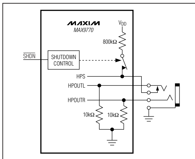
Figure 6. HPS Configuration
