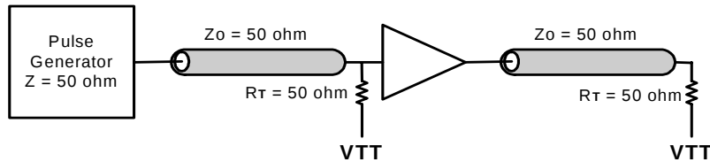
Figure 3. LVCMOS_CLK AC Test Reference for V_{DD} = 3.3\text{V}/2.5\text{V}
