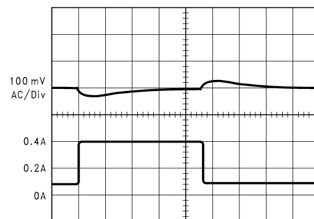
Figure 25. LM2674-3.3
