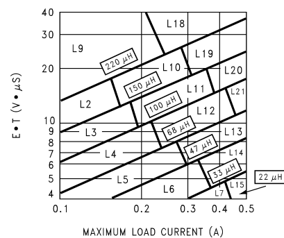
Figure 27. LM2674-ADJ
