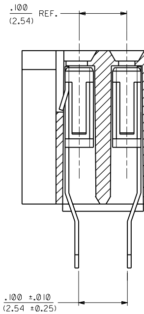
SECTION E-E
