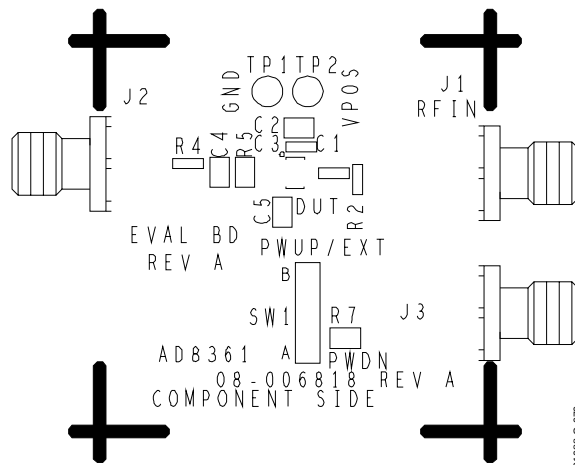
Figure 70. Silkscreen of the Component Side, SOT-23
