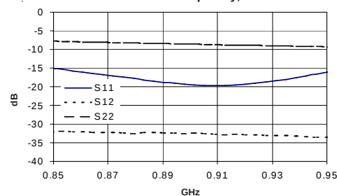
Input/Output Return Loss, Isolation vs. Frequency, T=25^\circ\text{C}
