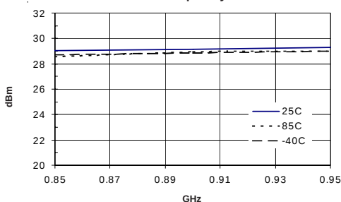
P1dB vs. Frequency
