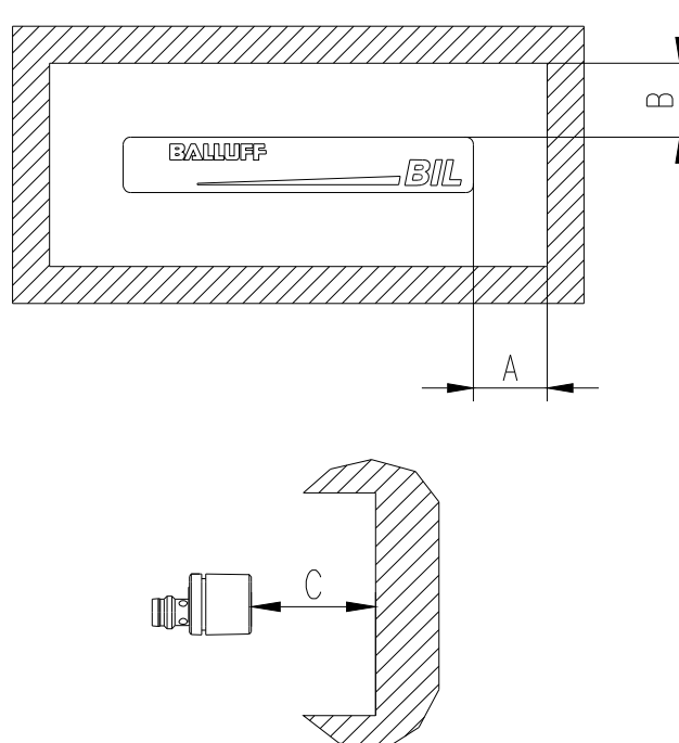
Installation diagram 2
