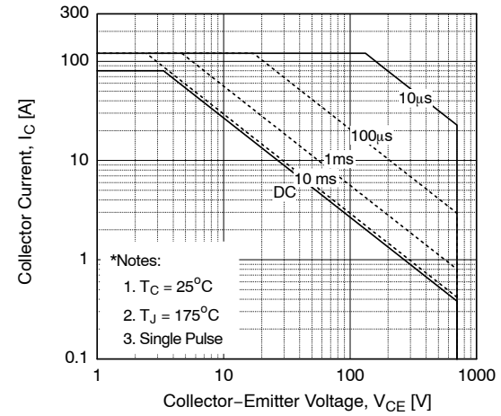
Figure 16. SOA Characteristics
