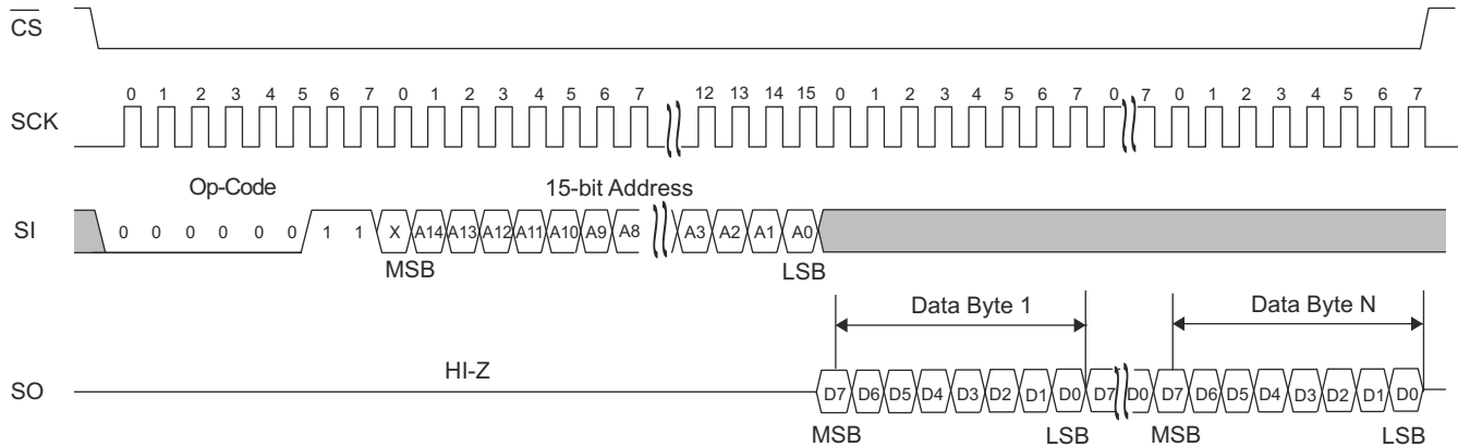
Figure 14. Fast Read Instruction Timing
