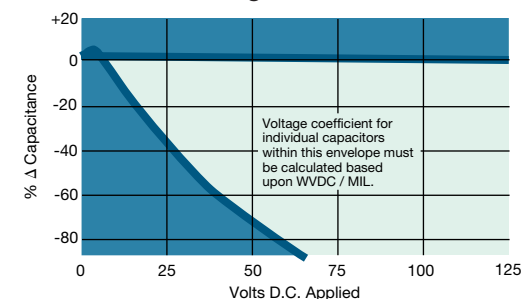
Voltage Coefficient
