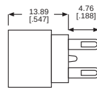
CONNECTOR 515-0074
