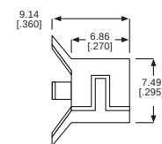
SPEED CLIP 515-0051
