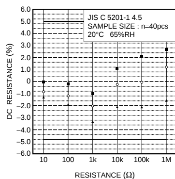
Fig.2 Resistance
