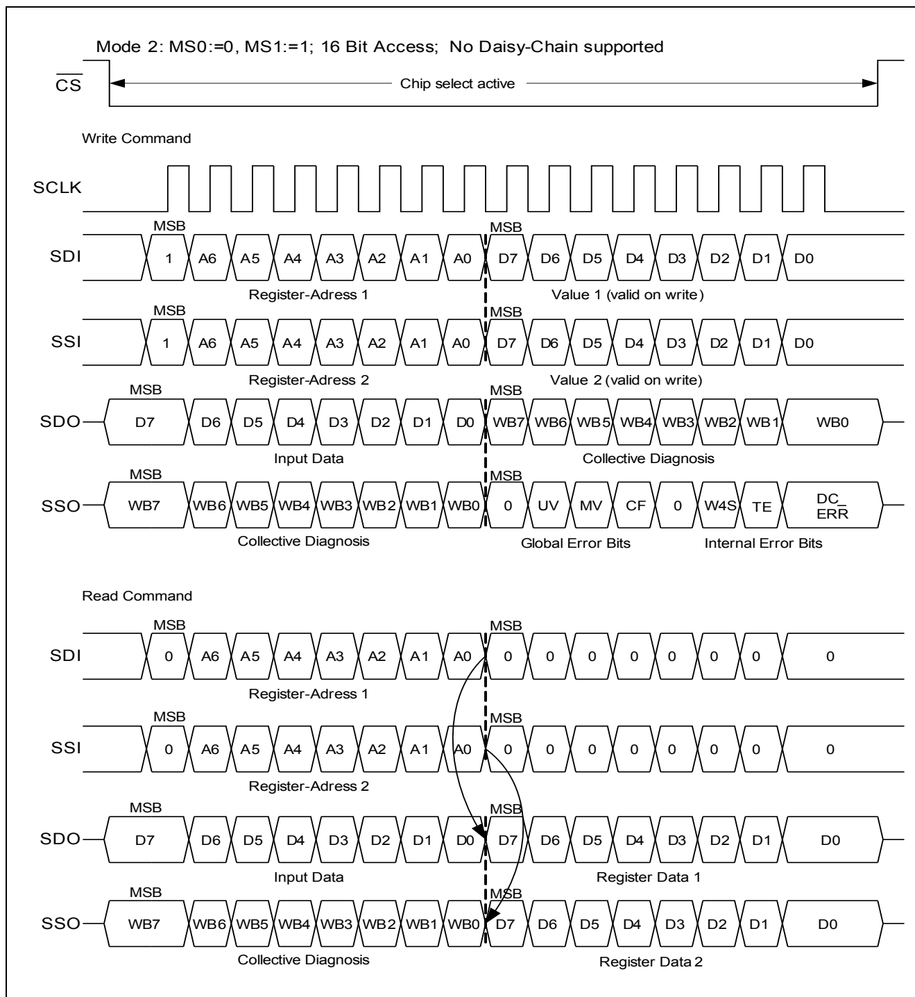
Figure 26 SPI Mode 2
