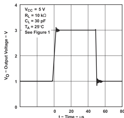
Figure 6-36. TLE2021 Voltage-Follower Large-Signal Pulse Response
