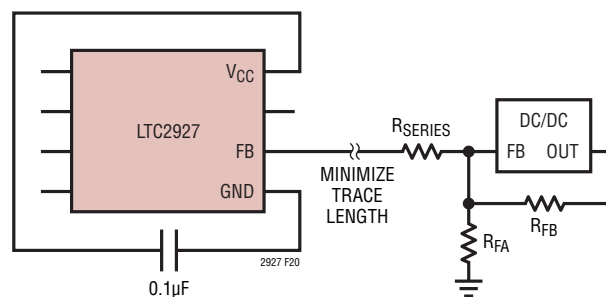
Figure 20. Layout Considerations
