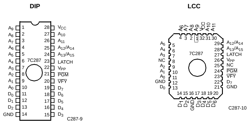
Figure 1. Programming Pinouts
