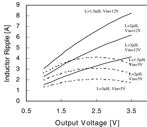
Figure 9. Inductor Ripple Current vs. Vout
