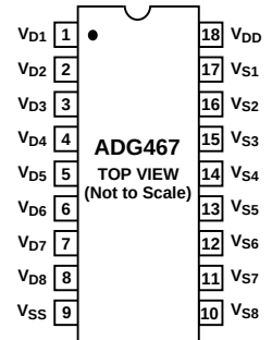
18-Lead SOIC
