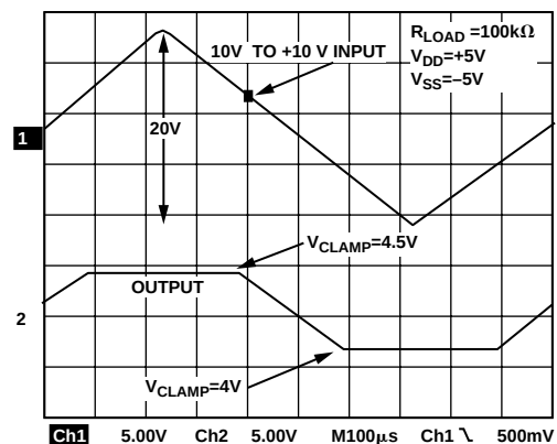
Figure 6. Overvoltage Ramp
