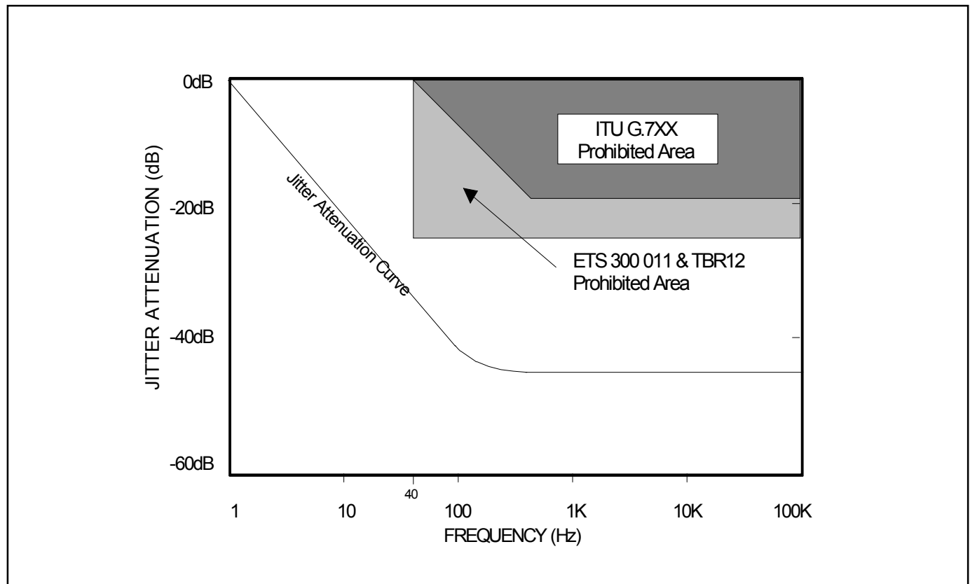
Figure 15-4. Jitter Attenuation
