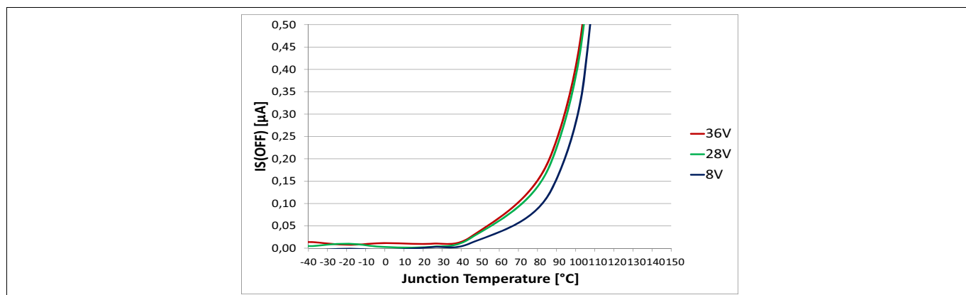
Figure 33 Standby Current for Whole Device with Load. I_{\text{S(OFF)}} = f(T_J; V_S)
