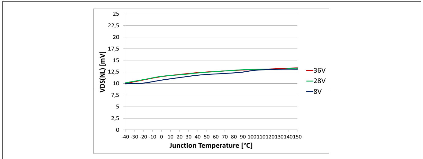
Figure 34 Output Voltage Drop Limitation at Low Load Current V_{DS(NL)} = f(T_J; V_S) ; I_L = I_{L(0)} = 50 \text{ mA}
