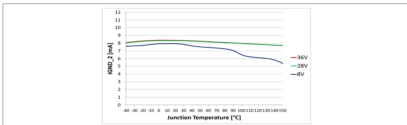
Figure 32 Current Consumption for Whole Device with Load. Two Channels Active I_{\text{GND}_2} = f(T_J; V_S)
