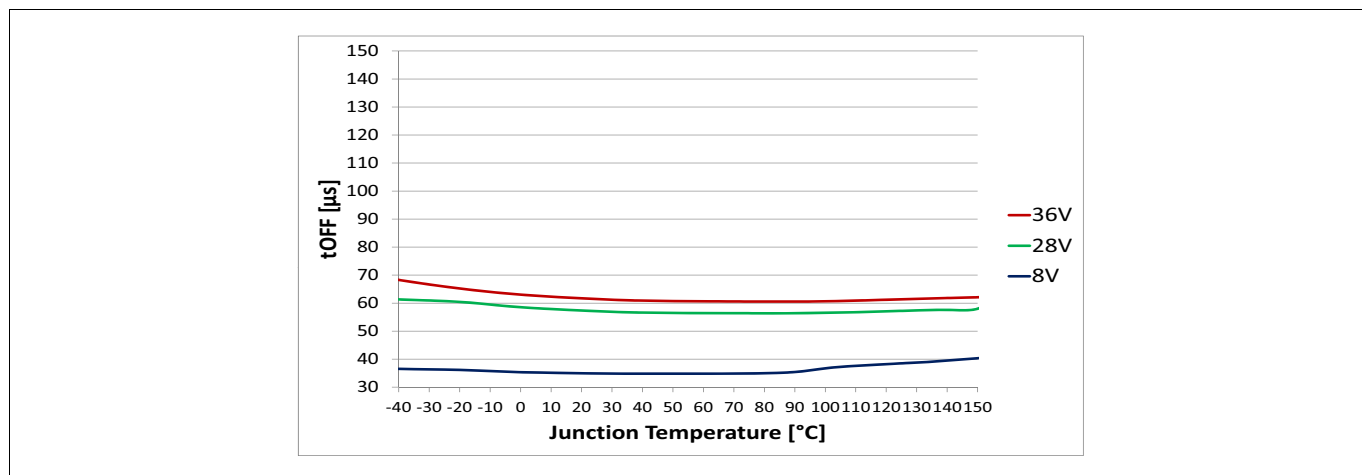
Figure 39 Turn OFF t_{\text{OFF}} = f(T_J; V_S) , R_L = 12 \Omega
