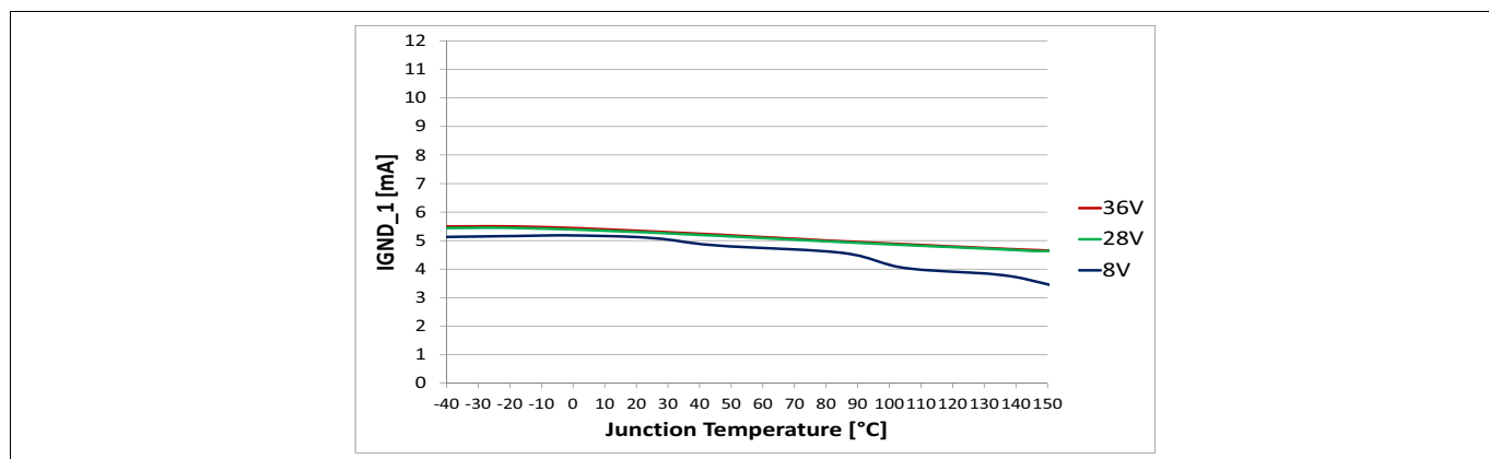
Figure 31 Current Consumption for Whole Device with Load. One Channel Active I_{\text{GND}_1} = f(T_J; V_S)
