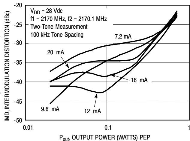
Figure 19. Intermodulation Distortion versus Output Power
