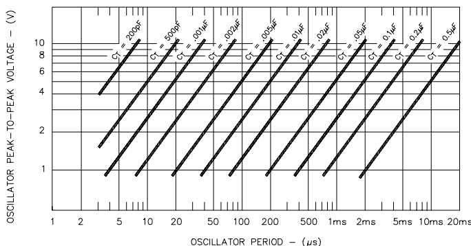
FIGURE 1 - SG1731 OSCILLATOR PERIOD VS. V_{DD} AND C.
