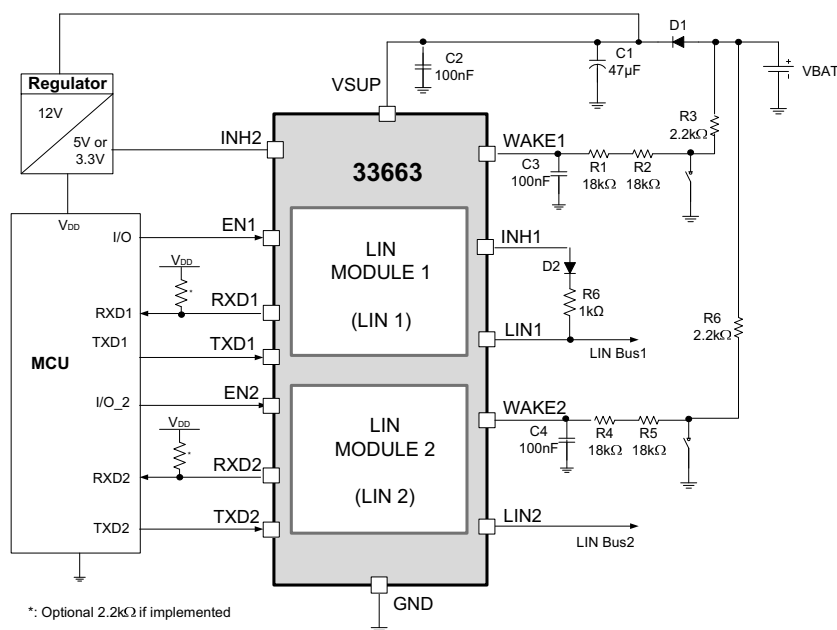
Figure 26. 33663 Typical Application
