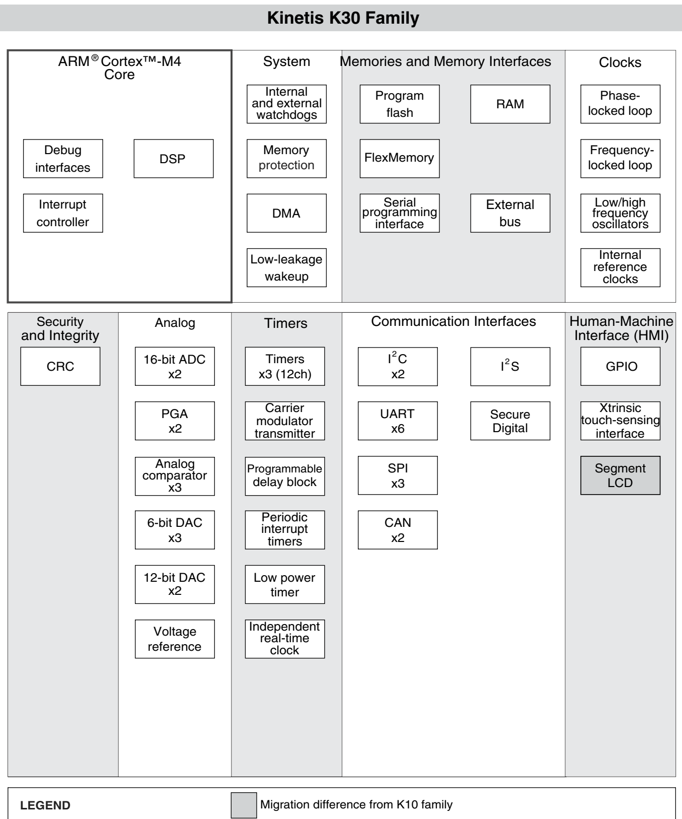
Figure 2. K30 Block Diagram
