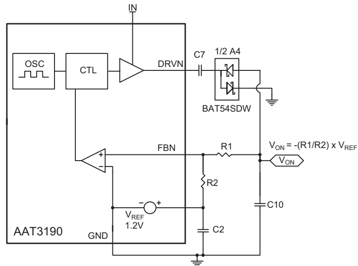
Figure 1: Negative Charge Pump Block Diagram
