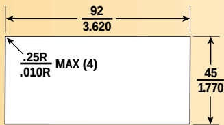
Panel Cutout
