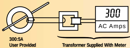
Connection for High Current Measurement
