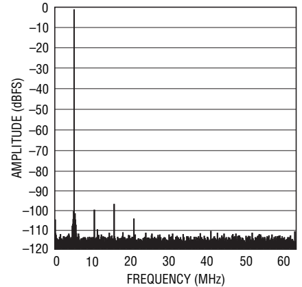
LTC2185: 64k Point FFT, f_{IN} = 5\text{MHz} , -1\text{dBFS} , 125Msps
