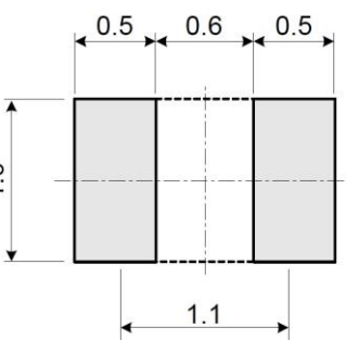
Figure 2) Suggested Land Pattern
