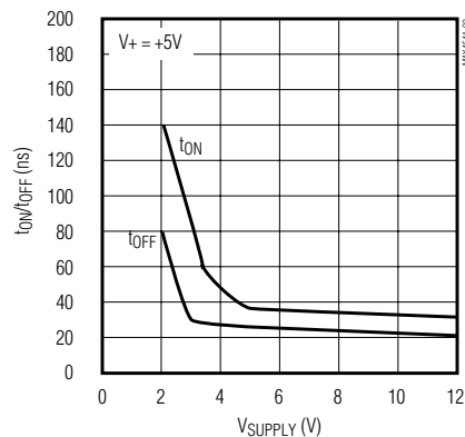
TURN-ON/OFF TIMES vs. SUPPLY VOLTAGE
