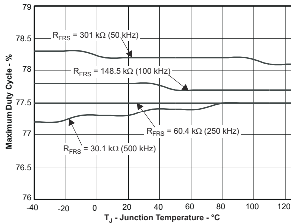
Figure 7-9. Maximum Duty Cycle vs Temperature
