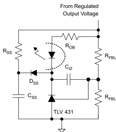
Figure 8-6. Example of Soft-Start Circuit Added to Error Amplifier
