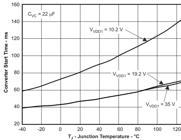
Figure 7-3. Converter Start Time vs Temperature
