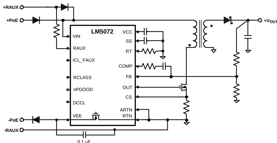
Figure 24. The RAUX Configuration
