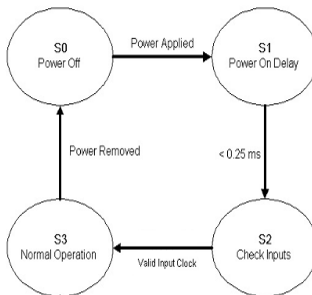
Figure 1. Buffer Power-up State Diagram
